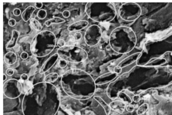
Figure 9 50/30/20 PP-EVA-PVA membrane treated with sandblasting. It showed larger pores and a higher size dispersion because of abrasion.
